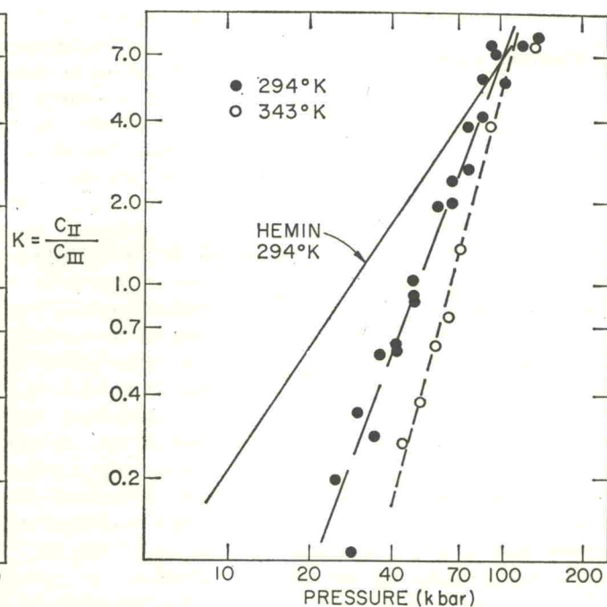
Fig. 7. \ln K vs. \ln P —Hematin
